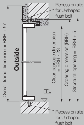
Door with stepped floor
