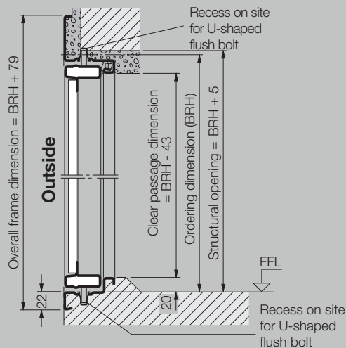
Door with flat floor
