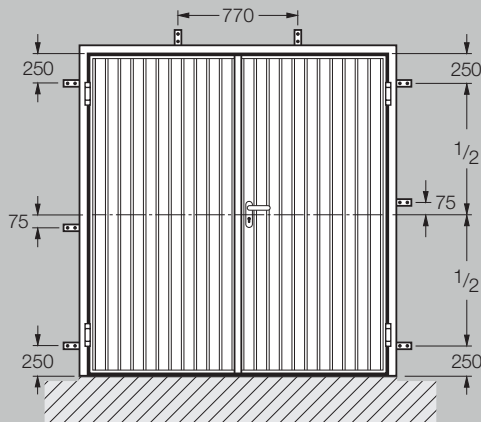
Position of anchors
